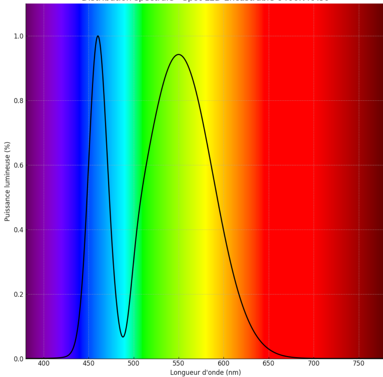
Distribution spectrale - Spot LED Encastrable 6400K RA80
