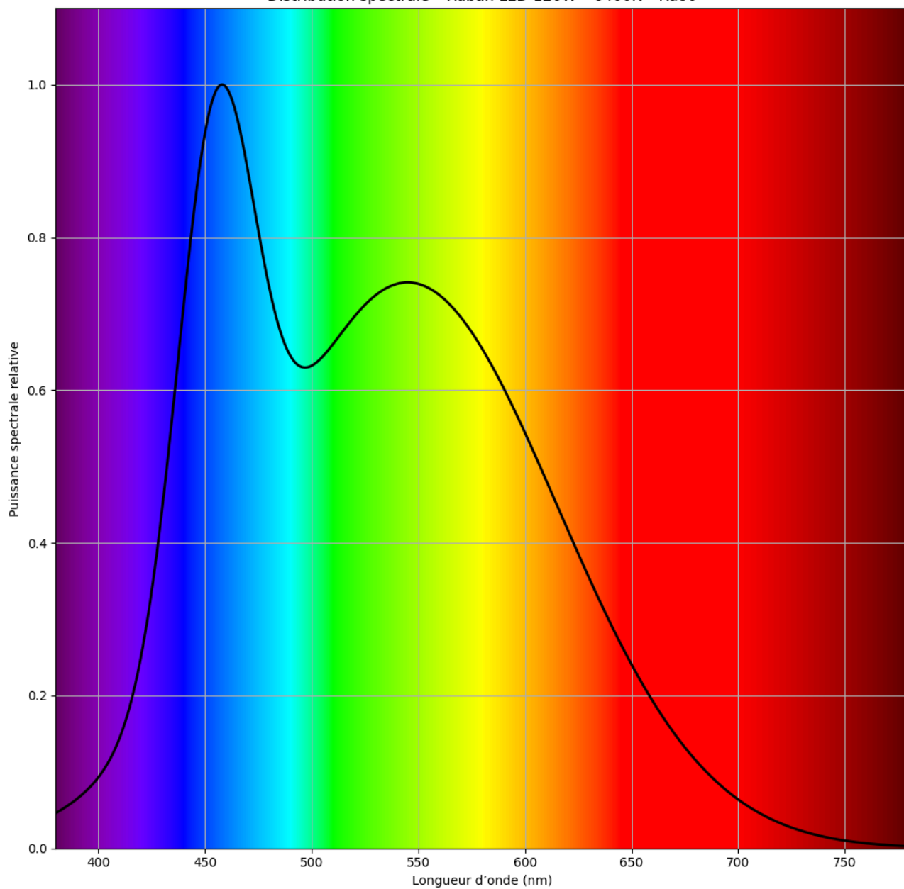
Distribution spectrale - Ruban LED 120W - 6400K - Ra80
