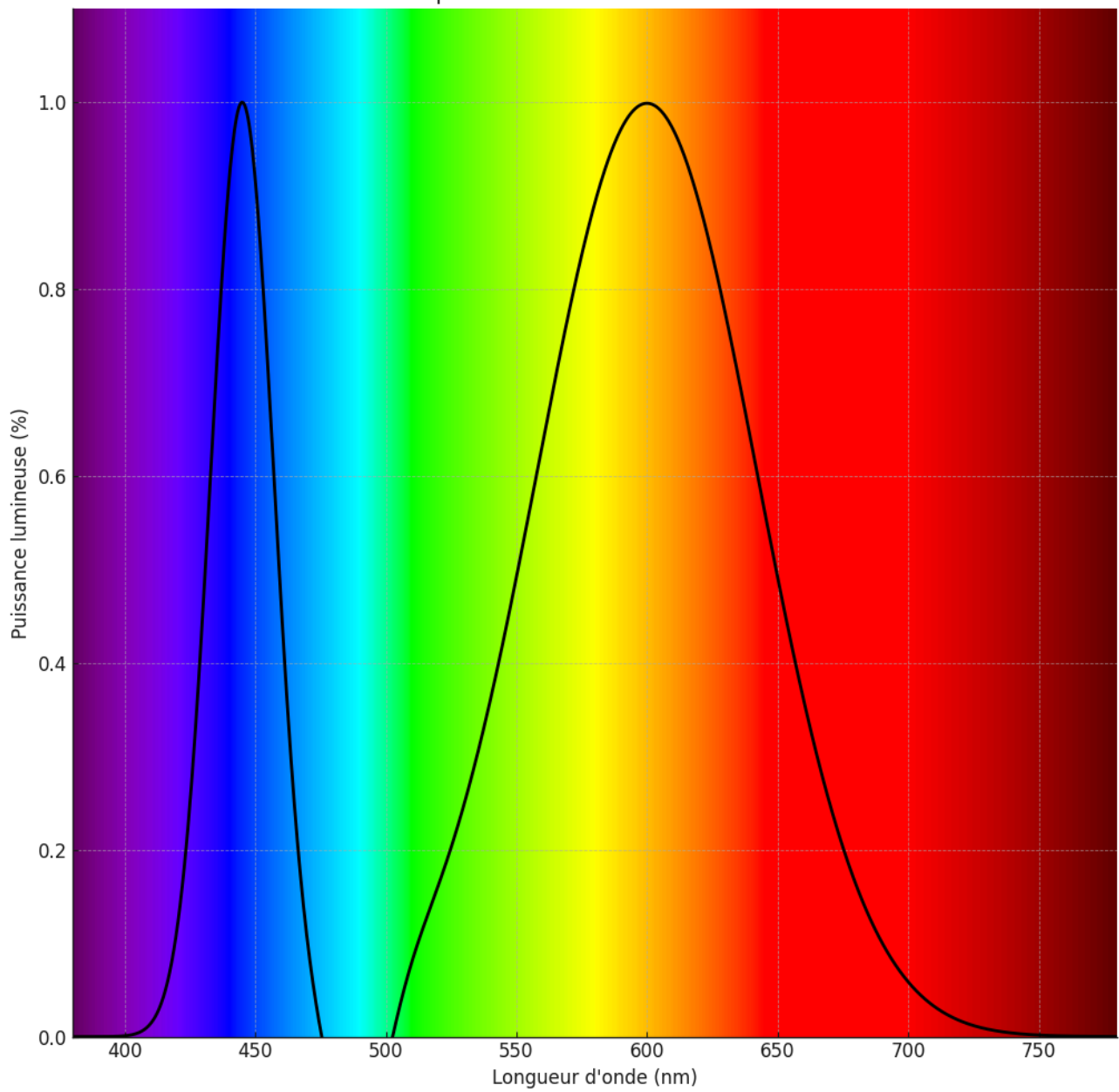
Distribution spectrale - Ruban LED 12W 3000K RA80
