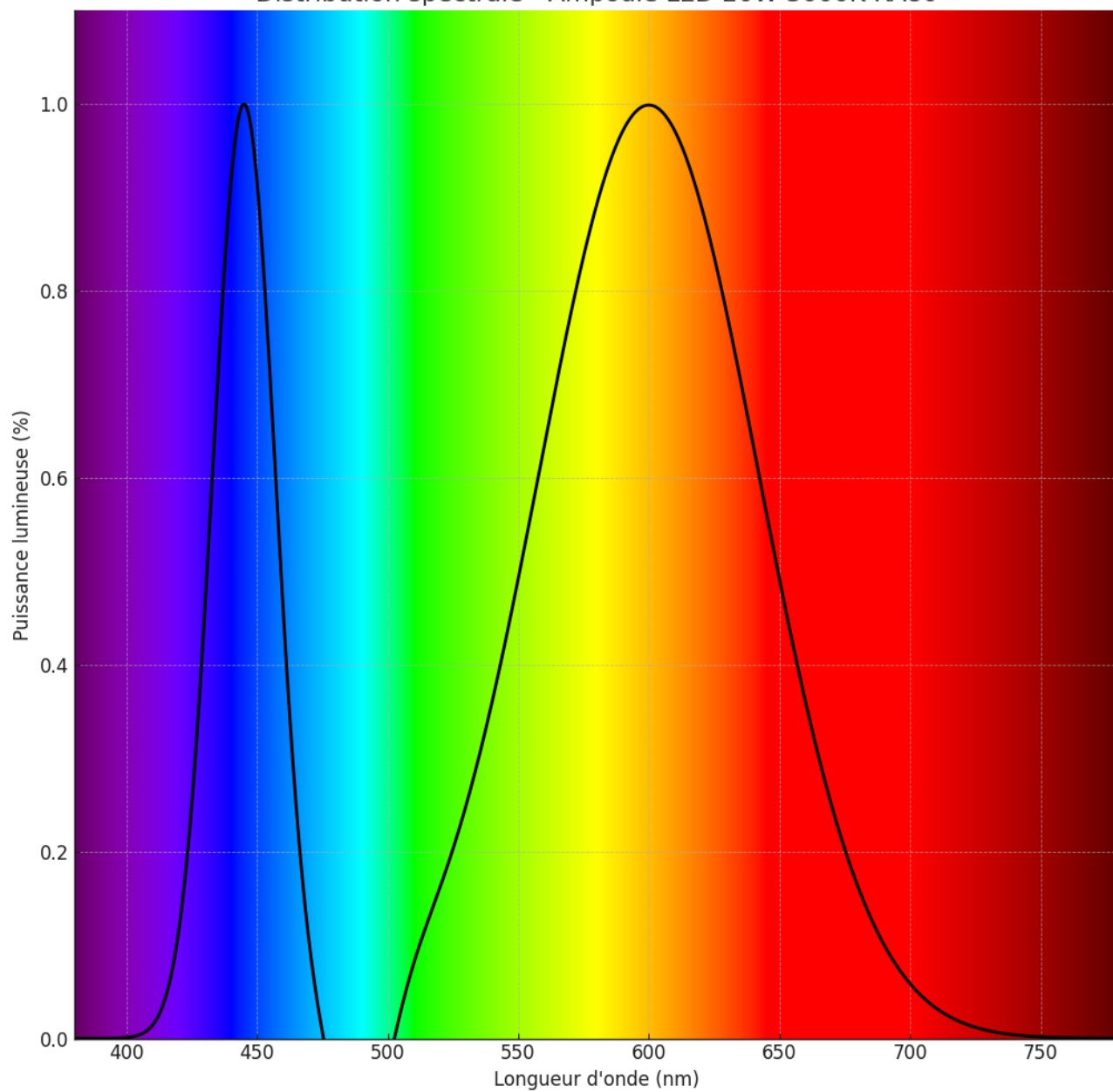
Distribution spectrale - Ampoule LED 20W 3000K RA80
