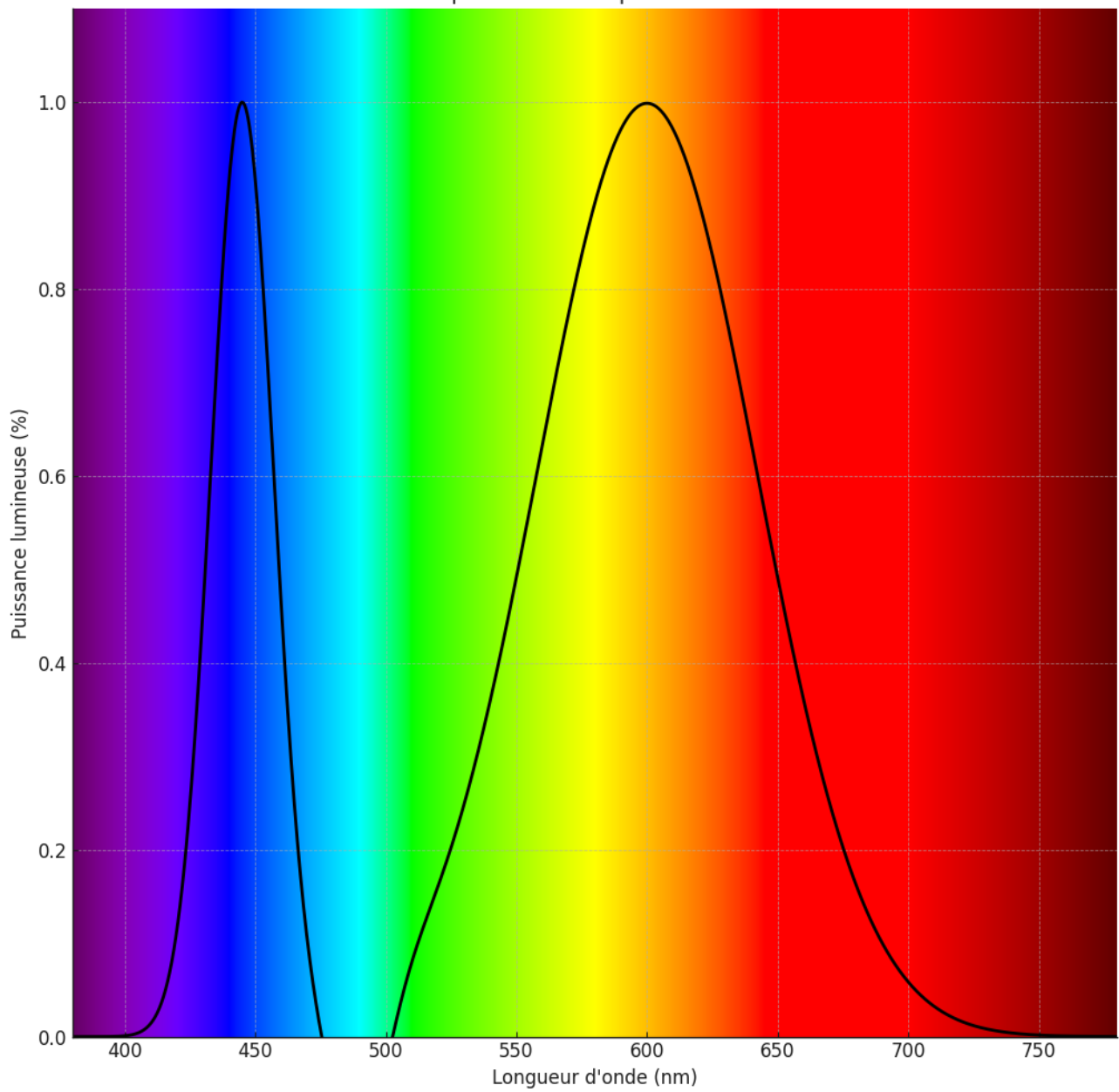
Distribution spectrale - Ampoule LED 3000K RA80
