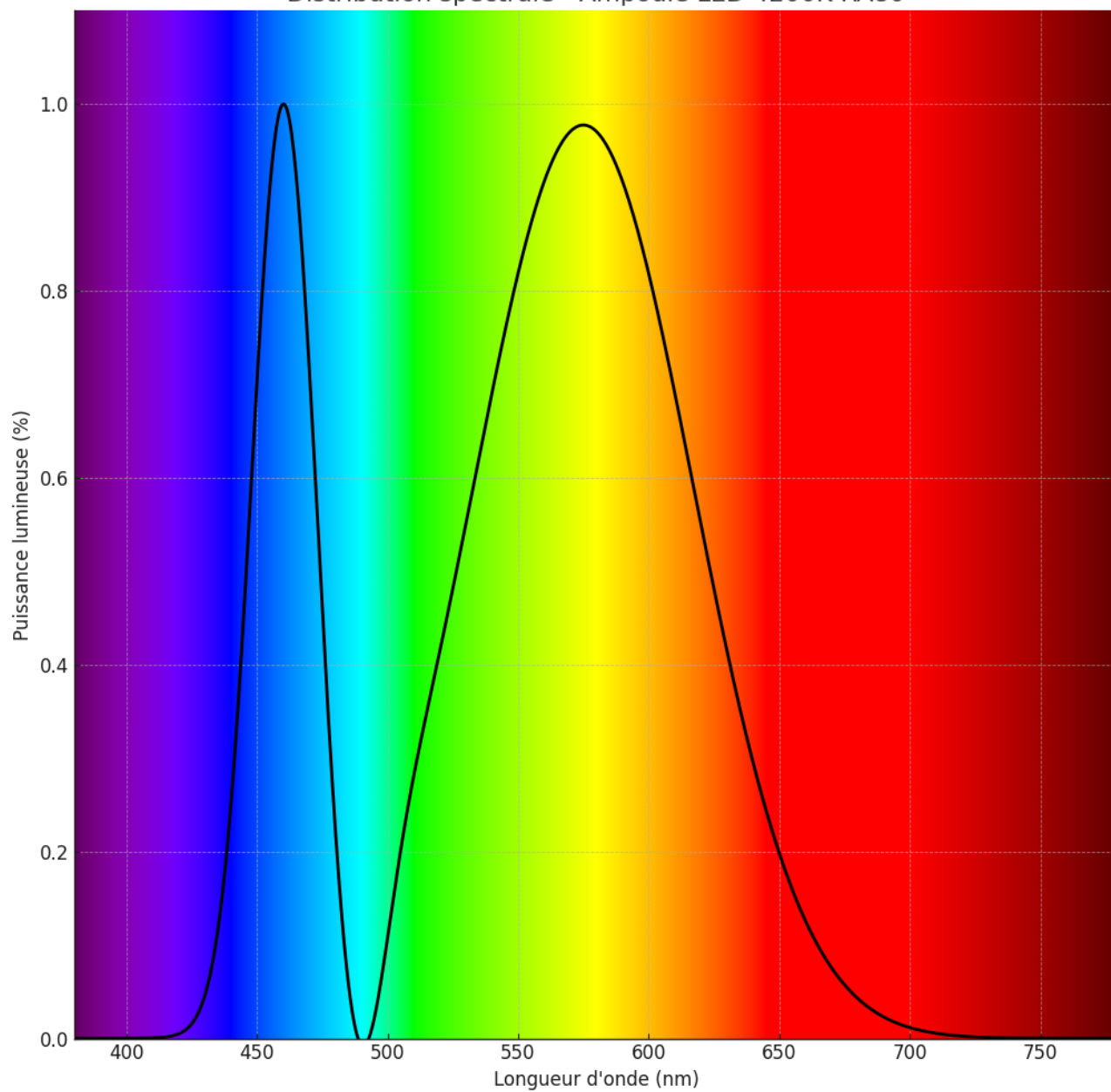
Distribution spectrale - Ampoule LED 4200K RA80
