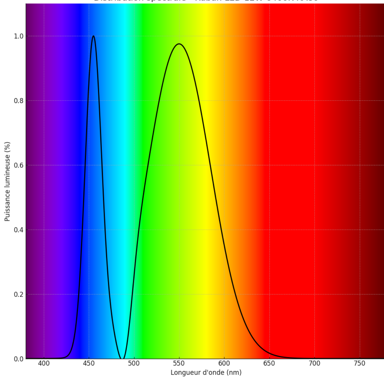
Distribution spectrale - Ruban LED 12W 6400K RA80
