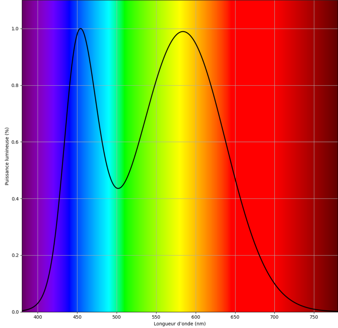
Distribution spectrale - Spot LED rond 9W CCT Ra80
