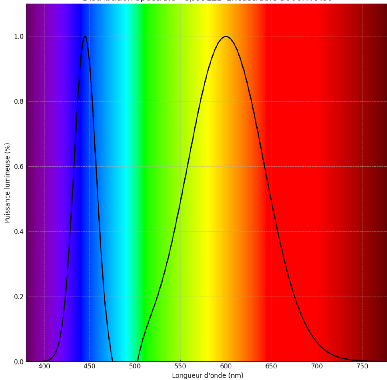
Distribution spectrale - Spot LED Encastrable 3000K RA80
