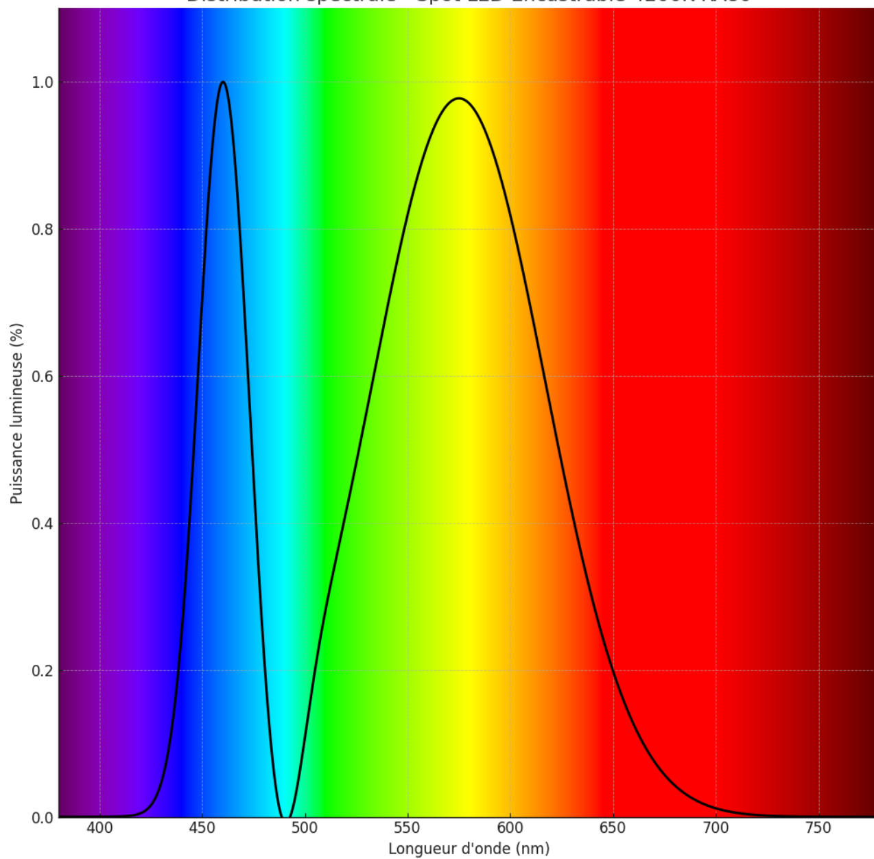
Distribution spectrale - Spot LED Encastrable 4200K RA80
