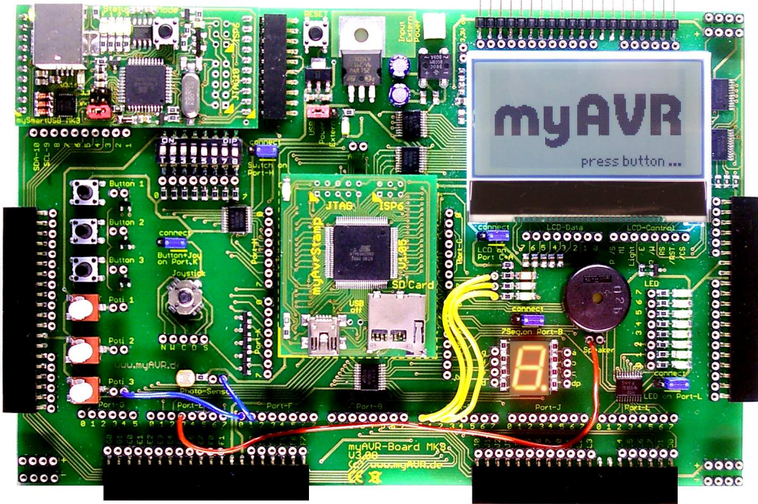
Abbildung / picture: myAVR Board MK3 / myAVR Board MK3
