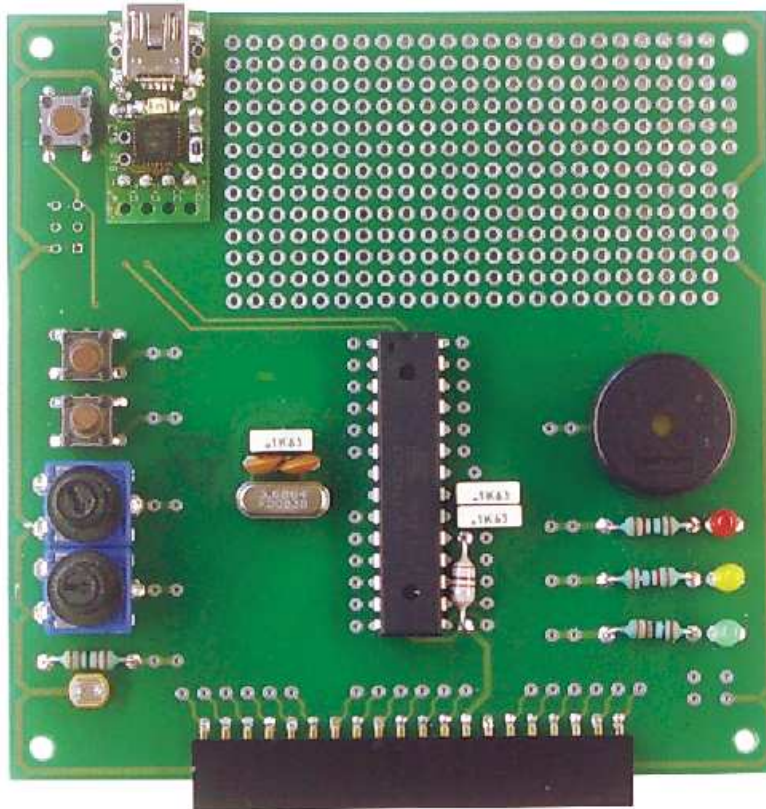
Assembled my AVR Board light
