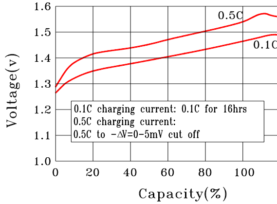
CHARGE CHARACTERISTICS
