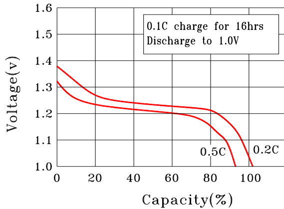
DISCHARGE CHARACTERISTICS
