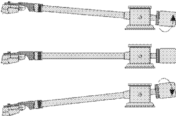
Fig. 4: Tone arm balance
