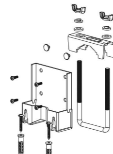
Mounting material
