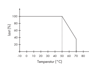
Abb. 5: Derating-Kurve
