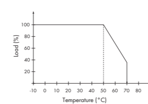
Fig. 5: Derating curve
