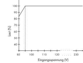
Abb. 6: Derating-Kurve
