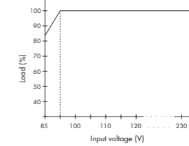
Fig. 6: Derating curve
