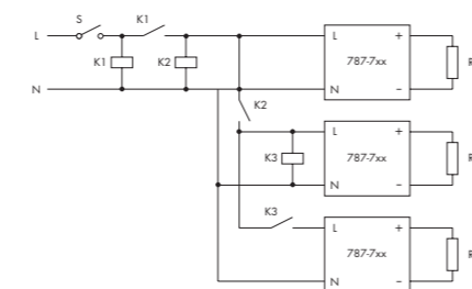
Fig. 3: Connecting power supply units in parallel
