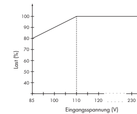
Abb. 6: Derating-Kurve
