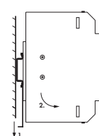
Fig. 2b: Disassembly
