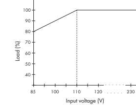
Fig. 6: Derating curve
