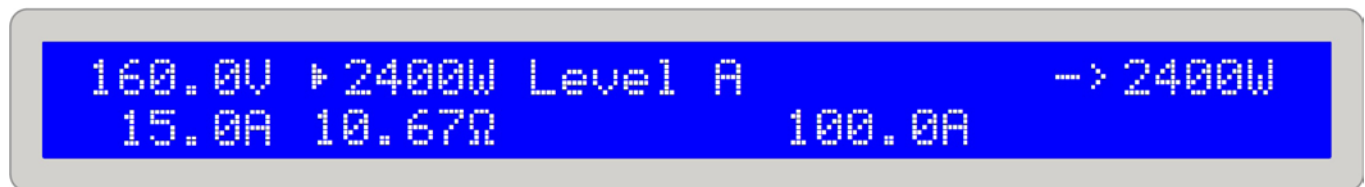
Figure 9. Normal load operation in CP regulation mode
