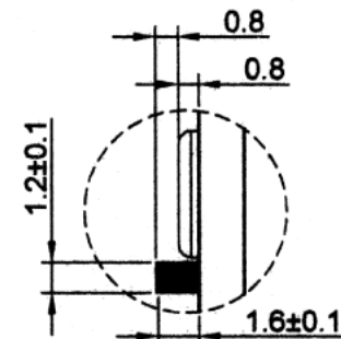
POLARITY PROTECTOR DEVICE DETAIL "A" S=3
