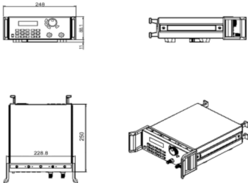
Fig.1-1 Dimension of SSL Load KONSTANTER Series 32 EL Programmable DC electronic load
