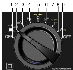
Figure 1: the switch
