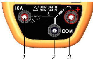
Figure 4: the terminals
