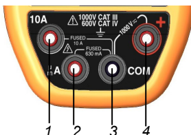
Figure 4: the terminals
