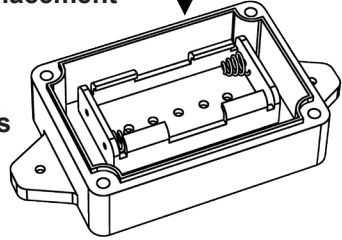
Fig. 1. Battery placement
