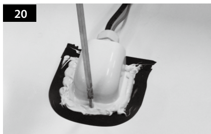
20 Fix cable holder on the car roof with 3 of M4x20 screws.
