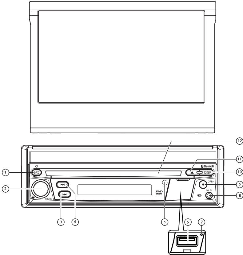
Figure 1. MAC 310 Controls and Indicators
