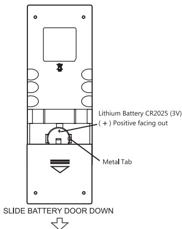
Figure 3. MAC 310 Remote Control Battery Replacement.
