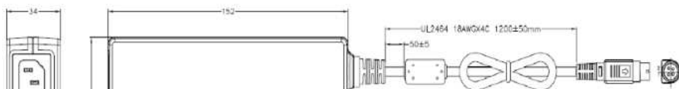
PSA120U-120L6
