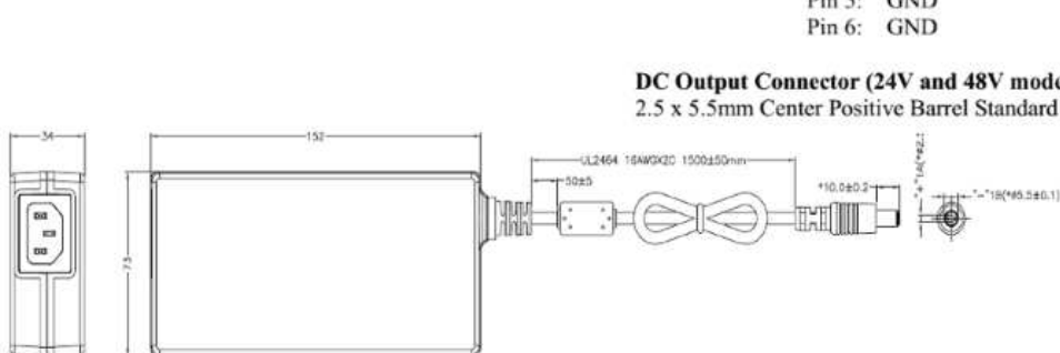
PSA120U-240L6, PSA120U-480L6
