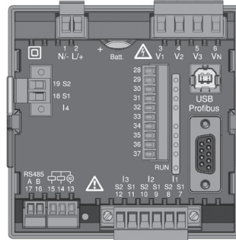
Fig. Rear side view of UMG 96 RM-P
