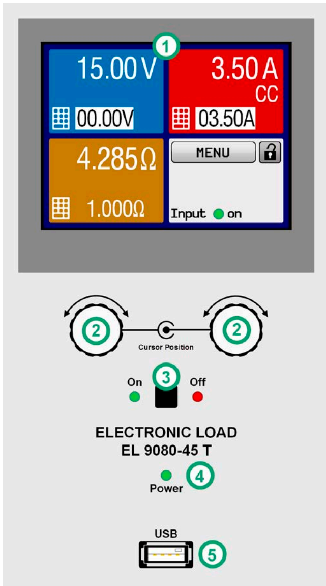
Figure 5 - Control Panel
