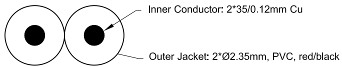
Cable Structure
