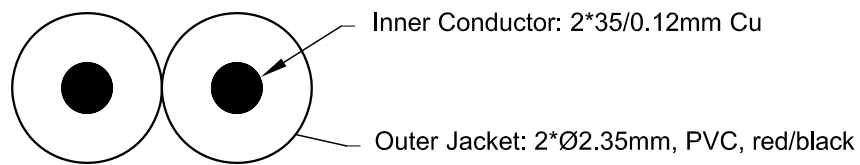
Cable Structure
