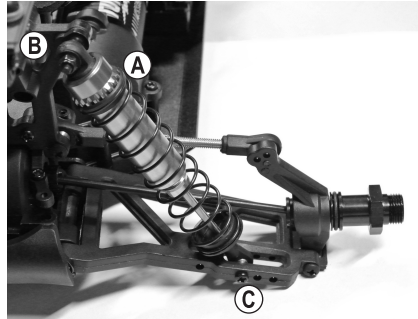
Rear axle
