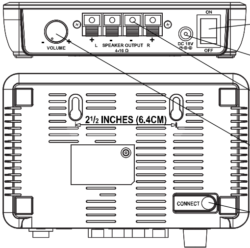
Surround Anywhere 221 audio receiver
