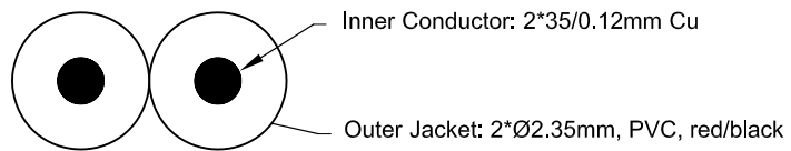
Cable Structure
