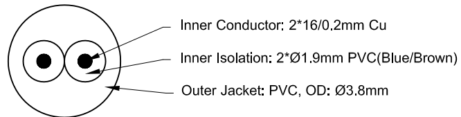
Cable Structure (0.5mm 2 )
