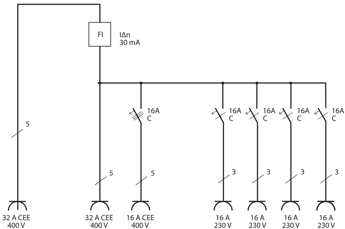
Afb. F: Wandverdeler WV 4/32A IP44
