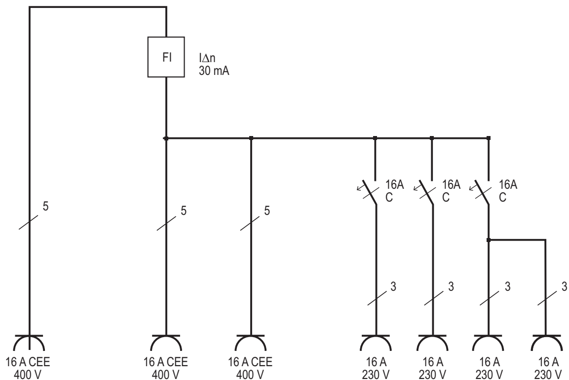
Fig. E: WV 4/16 A IP44 distribution box
