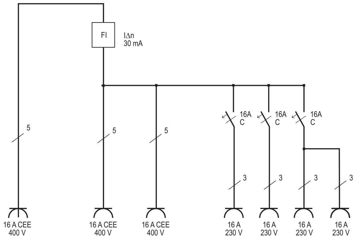
Afb. E: Wandverdeler WV 4/16A IP44
