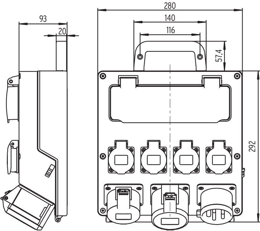
Fig. D: Housing dimensions
