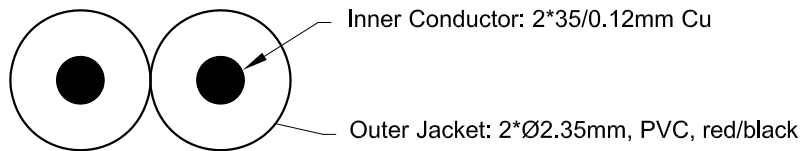
Cable Structure
