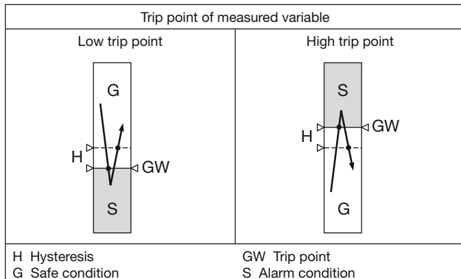
Fig. 4. Switching function, according to trip point type.
