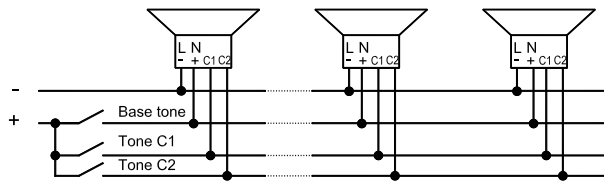
Connection example
