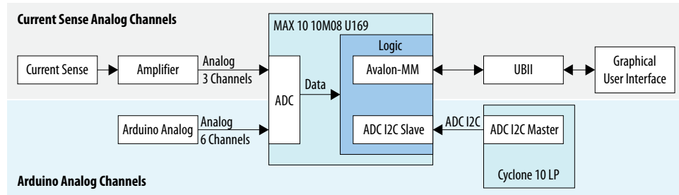
Figure 13. Current Measurement
