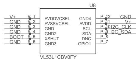
Figure 4. STEVAL-BCN002V1 schematic (2 of 3)
