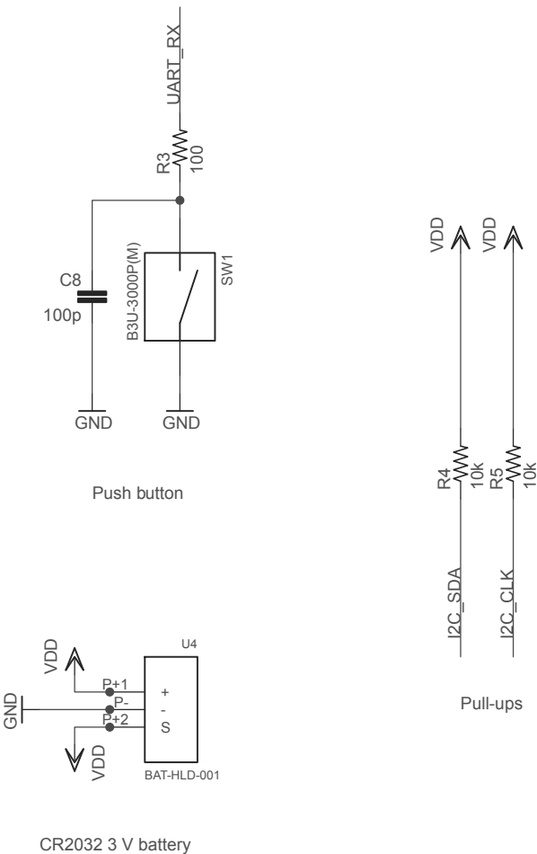
Figure 5. STEVAL-BCN002V1 schematic (3 of 3)
