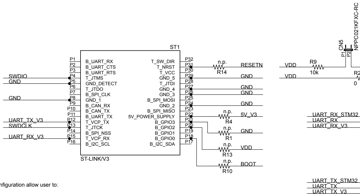
Figure 8. STEVAL-BCN002V1D schematic (3 of 3)
