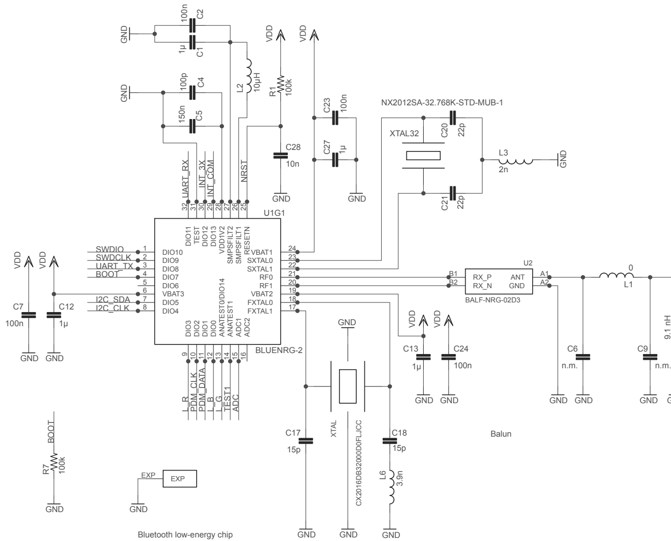
Figure 3. STEVAL-BCN002V1 schematic (1 of 3)
