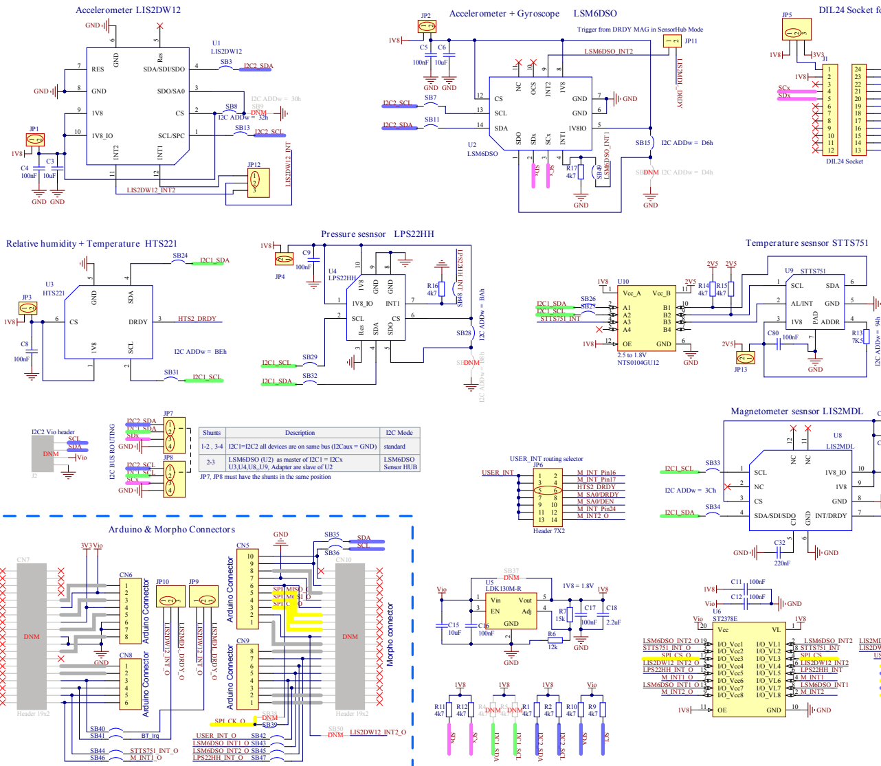
Figure 8. X-NUCLEO-IKS01A3 board schematics
