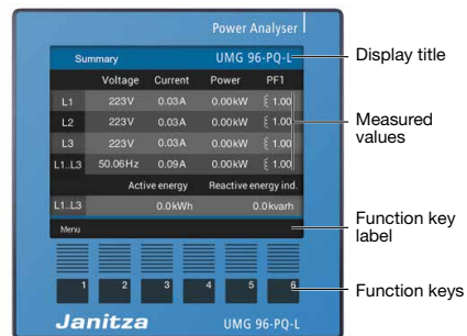
Fig. UMG 96-PQ-L standard display - measured values display "Summary"
