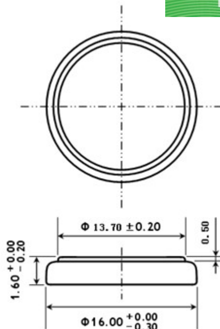
Dimension Drawing
