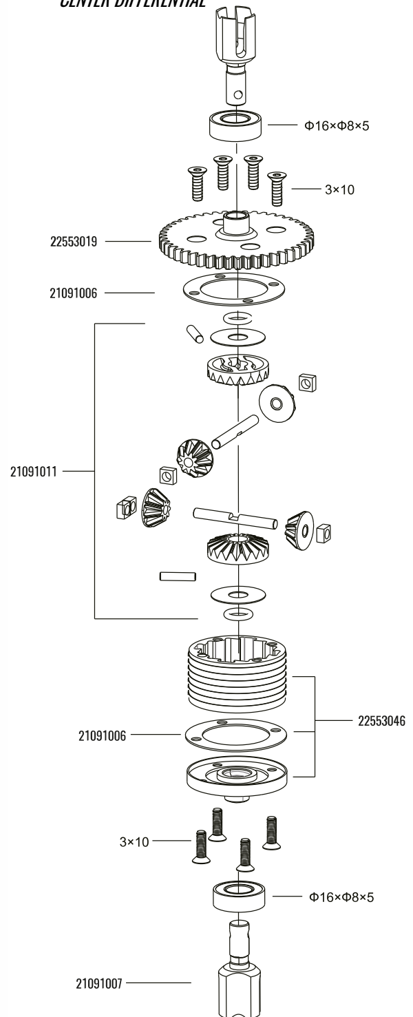
MITTEL-DIFFERENTIAL CENTER DIFFERENTIAL
