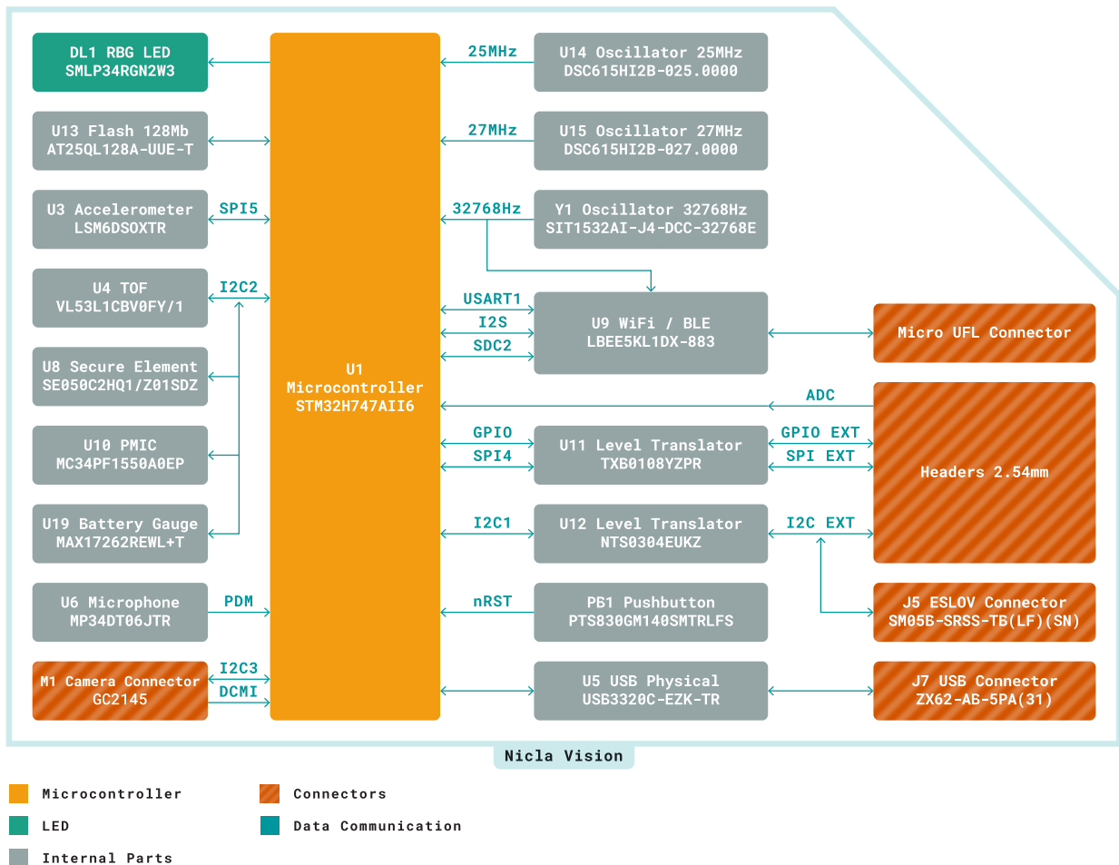
Nicla Vision Block Diagram
