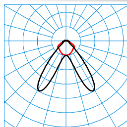
C-Line DA-25 LED4000-830 TX055249
