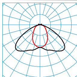
C-Line XB LED12000-830 TX055471
