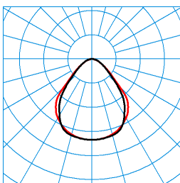
PareliaAct H-L 13000 +LM3 03 N8 (ActDCW) (LEO_direct_c270geo) TX121931 ■ C0 - C180 ■ C90 - C270 UGR I = 18,4 UGR q = 17,3 DIN 5040: A50 UTE: 1,00 C CEN Flux Code: 66 90 98 100 100 0 0 0 0
