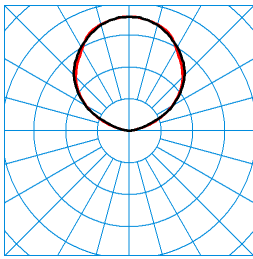
PareliaAct H-L 13000 +LM1 03 N8 (ActDSU) (LEO_indirect) TX121980 ■ C0 - C180 ■ C90 - C270 DIN 5040: E03 UTE: 0,00 J + 1,00 T CEN Flux Code: 0 0 0 0 100 48 82 97 100
