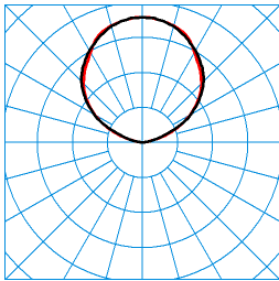
PareliaAct H-L 13000 +LM1 03 N8 (ActDCW) (LEO_indirect) TX121877 ■ C0 - C180 ■ C90 - C270 DIN 5040: E03 UTE: 0,00 J + 1,00 T CEN Flux Code: 0 0 0 0 100 48 82 97 100
