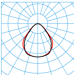
PareliaAct H-L 13000 +LM2 03 N8 (ActDCW) (LEO_direct_c90geo) TX121957 ■ C0 - C180 ■ C90 - C270 UGR I = 18,4 UGR q = 17,3 DIN 5040: A50 UTE: 1,00 C CEN Flux Code: 66 90 98 100 100 0 0 0 0
