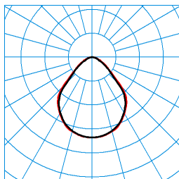
Parelia H-LM 11500-840 01 (direct c90geo) TX057106 ■ C0 - C180 ■ C90 - C270 UGR I = 18,5 UGR q = 17,2 DIN 5040: A50 UTE: 1,00 C CEN Flux Code: 65 91 99 100 100
