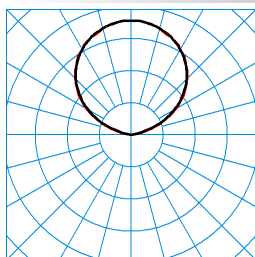
Parelia H-LM 11500-840 01 (indirect) TX057107 ■ C0 - C180 ■ C90 - C270 DIN 5040: E03 UTE: 0,00 J + 1,00 T CEN Flux Code: 0 0 0 0 100 49 82 98 100
