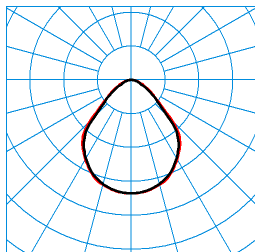
Parelia H-LM 11500-840 01 (direct c270geo) TX057105 ■ C0 - C180 ■ C90 - C270 UGR I = 18,5 UGR q = 17,2 DIN 5040: A50 UTE: 1,00 C CEN Flux Code: 65 91 99 100 100
