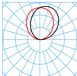
Sanesca W3 LED5000-840 01 (night light) TX055769
