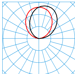
Sanesca W3 LED5000-840 01 (room light) TX055771
